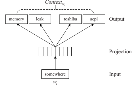
Fig. 2. An example of skip-gram model.
